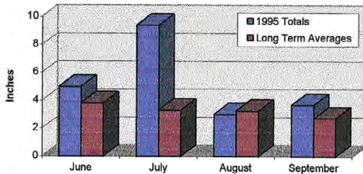
Figure 6. Precipitation Comparison
